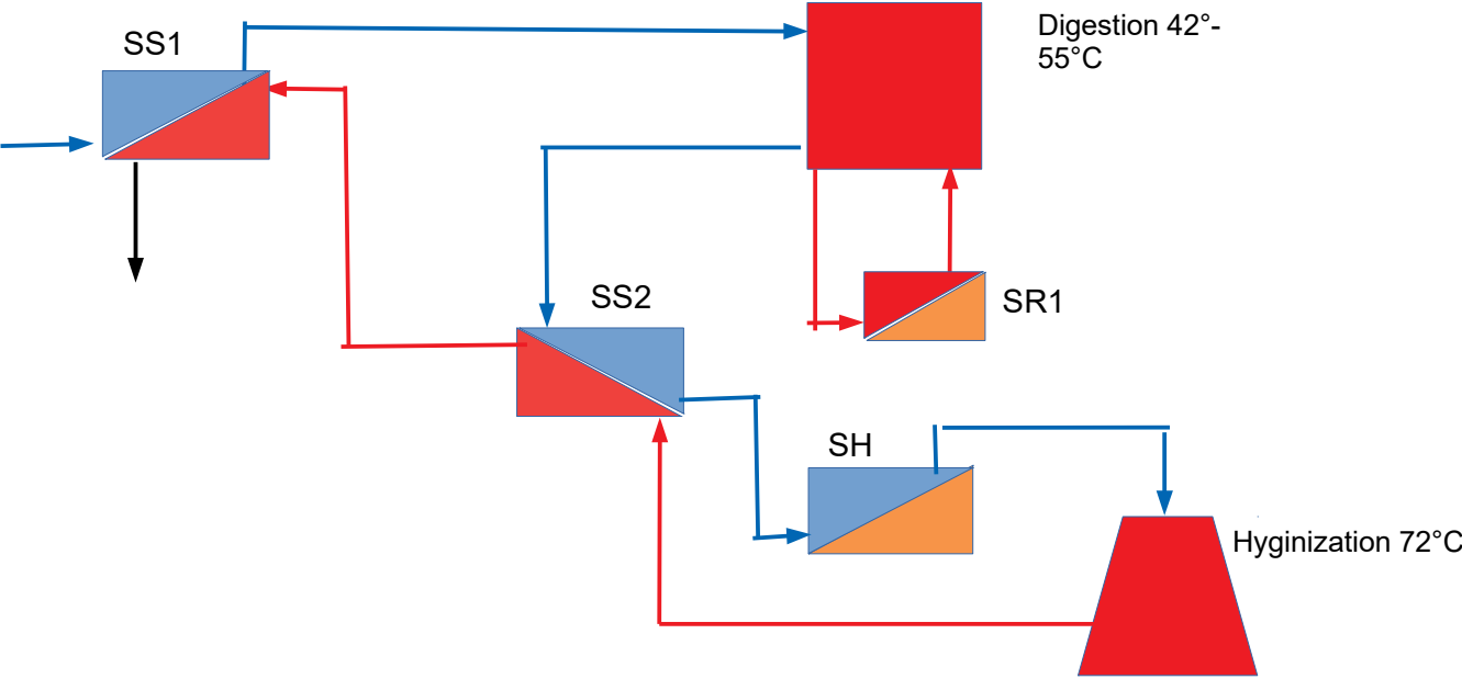
System with hyginization after digestion.
