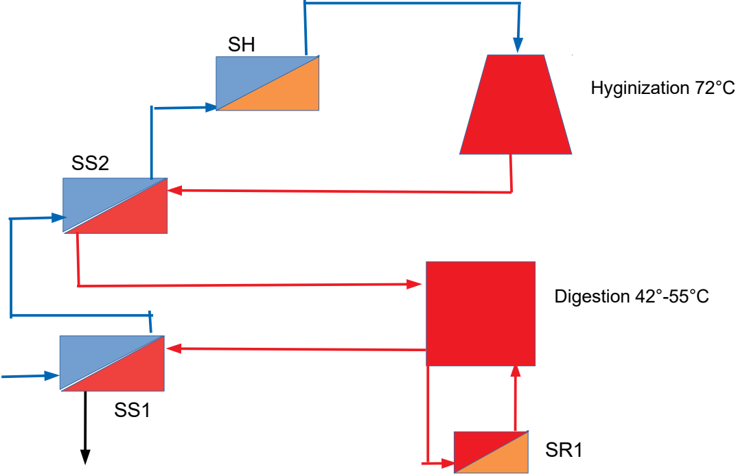
System with hyginization before digestion.
