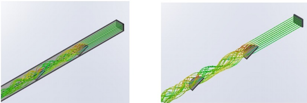
Forced stirring. (Software simulation situation using sludge and design data).
